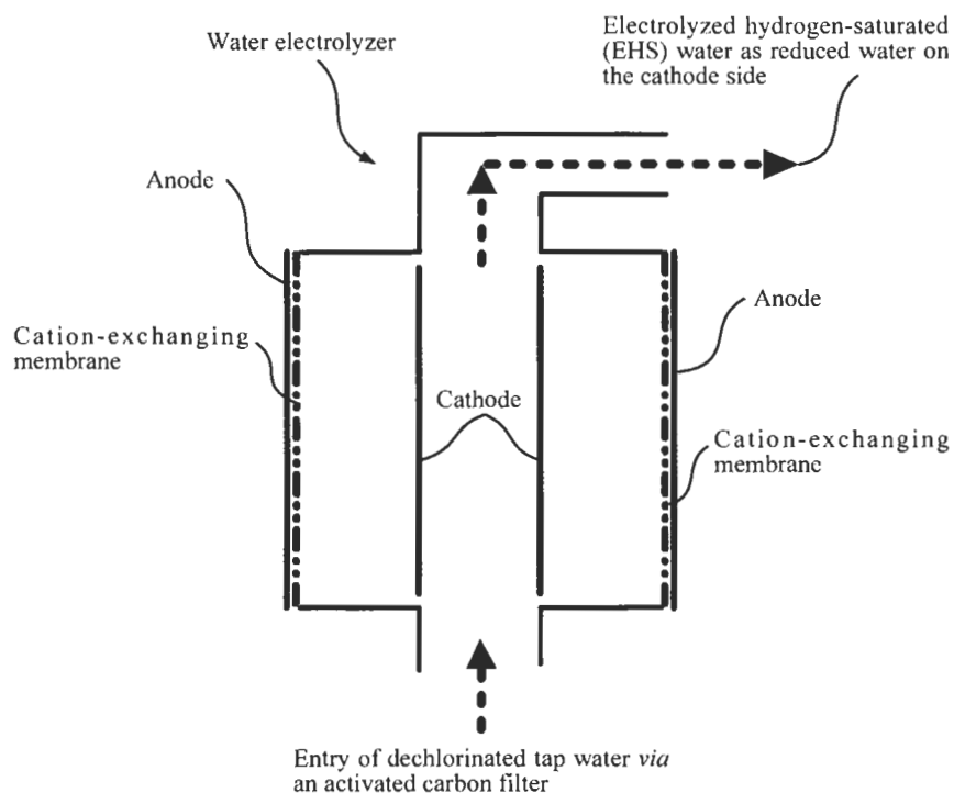
Fig. 1. Device for Use in Producing Electrolyzed Hydrogen-Saturated Water.
